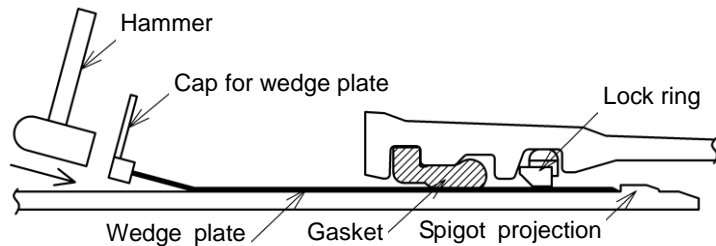
Fig.-46 Pushed wedge plate into socket
