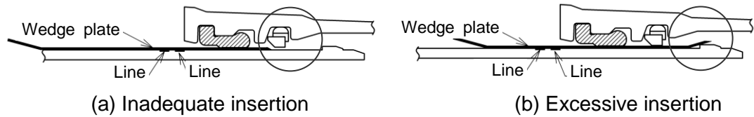
Fig.-47 Improper insertion of wedge plate
