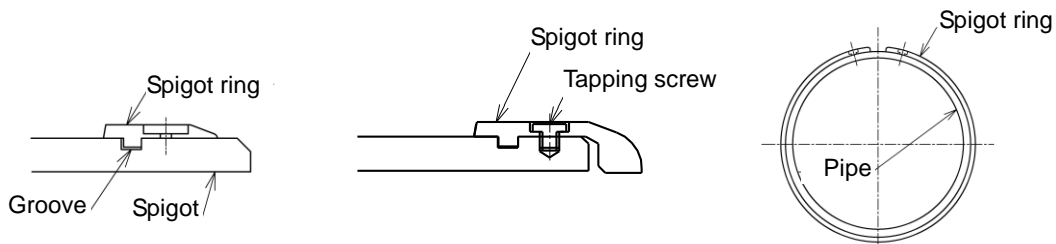
Fig.-39 Spigot ring set on the spigot end
