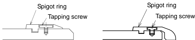
Fig.-43 Spigot ring installed with Tapping screw
