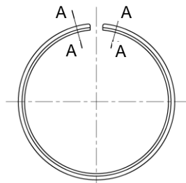
Fig.-37 Spigot ring for cut pipe
